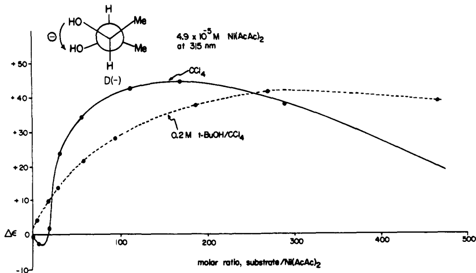
Figure 4. Variation of \Delta\epsilon at 315 nm for \text{Ni}(\text{acac})_2 ( 4.9 \times 10^{-5} M ) with increasing concentrations of (2 R ,3 R )-butane-2,3-diol in \text{CCl}_4 (—) and in 0.2 M t -BuOH- \text{CCl}_4 (---).
