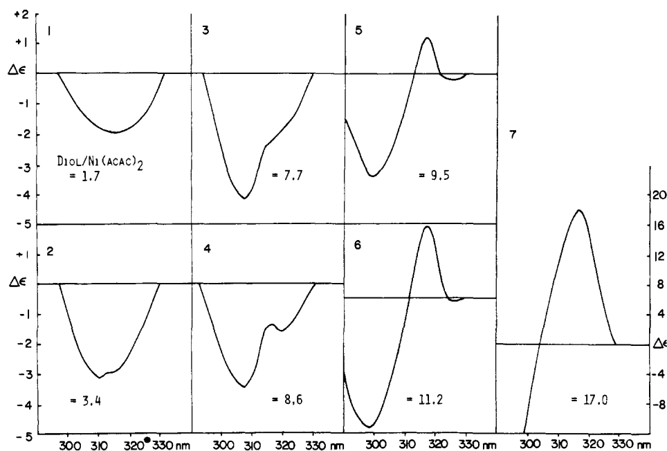
Figure 5. The CD of a mixture of \text{Ni}(\text{acac})_2 ( 7.0 \times 10^{-5} M ) and increasing concentrations of (2R,3R) -butane-2,3-diol. The molar ratios of diol/Ni are: (1) 1.7:1; (2) 3.4:1; (3) 7.7:1; (4) 8.6:1; (5) 9.5:1; (6) 11.2:1; and (7) 17.0:1.
