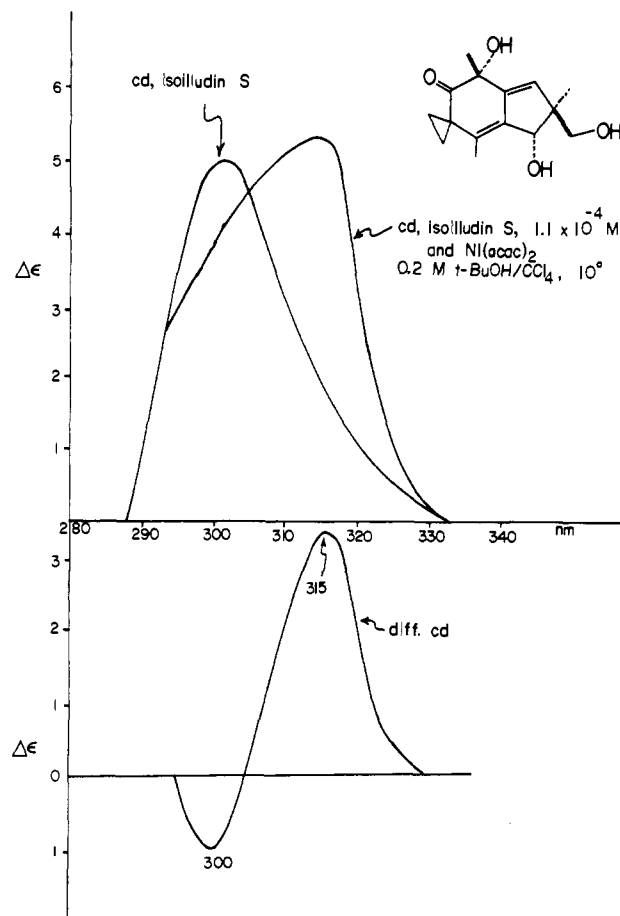
Figure 11. The CD of isoilludin S ( 1.1 \times 10^{-4} M ) and that with Ni(acac) 2 added as a solid (ca. 5 \times 10^{-5} M ), in a solution of 0.2 M t -BuOH-CCl 4 at 10°. Lower trace is the difference curve.
