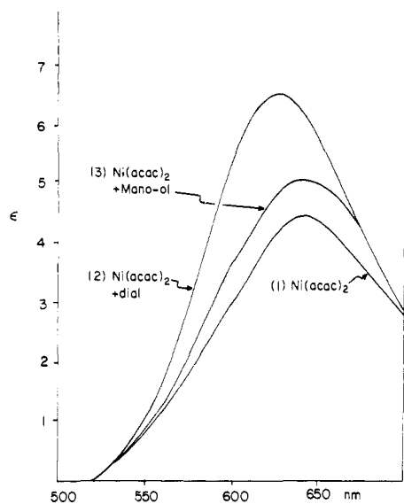
Figure 2. The uv, in \text{CCl}_4 , of: (1) an 8.33 \times 10^{-4} M solution of \text{Ni}(\text{acac})_2 ; (2) a mixture of 8.33 \times 10^{-4} M \text{Ni}(\text{acac})_2 and 3.33 \times 10^{-2} M (2R,3R) -butane-2,3-diol; (3) a mixture of 8.33 \times 10^{-4} M \text{Ni}(\text{acac})_2 and 3.33 \times 10^{-2} M (2R) -3-methylbutan-2-ol.
