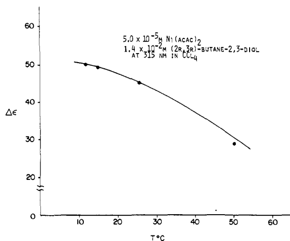
Figure 8. Variation of \Delta\epsilon at 315 nm with temperature for a mixture of \text{Ni}(\text{acac})_2 ( 5.0 \times 10^{-5} M ) and (2R,3R) -butane-2,3-diol ( 1.4 \times 10^{-2} M ) in \text{CCl}_4 .
