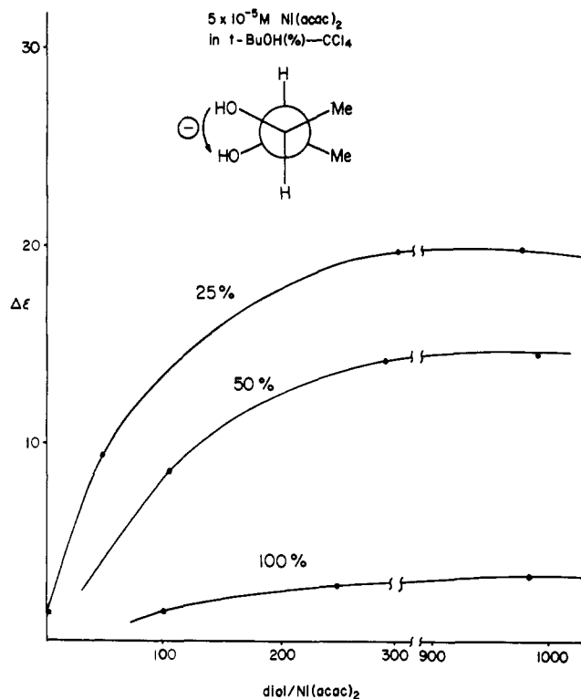
Figure 10. Variation of the CD observed at 315 nm for a \text{Ni}(\text{acac})_2 ( 5 \times 10^{-5} M ) solution with increasing concentrations of (2R,3R) -butane-2,3-diol in 25% t -BuOH- \text{CCl}_4 , 50% t -BuOH- \text{CCl}_4 and 100% t -BuOH solutions.
