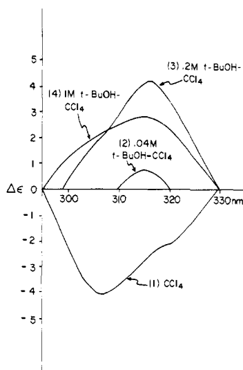
Figure 6. Curve 1: CD of a mixture of \text{Ni}(\text{acac})_2 ( 7.0 \times 10^{-5} M ) and (2R,3R) -butane-2,3-diol ( 5.0 \times 10^{-4} M ) in \text{CCl}_4 . Curve 2: CD of a mixture of \text{Ni}(\text{acac})_2 ( 4.0 \times 10^{-5} M ) and the diol ( 2.8 \times 10^{-4} M ) in a 0.04 M t -BuOH- \text{CCl}_4 solution. Curve 3: same mixture as in curve 2, in a 0.2 M t -BuOH- \text{CCl}_4 solution. Curve 4: same mixture as in curve 2, in a 1 M t -BuOH- \text{CCl}_4 solution.
