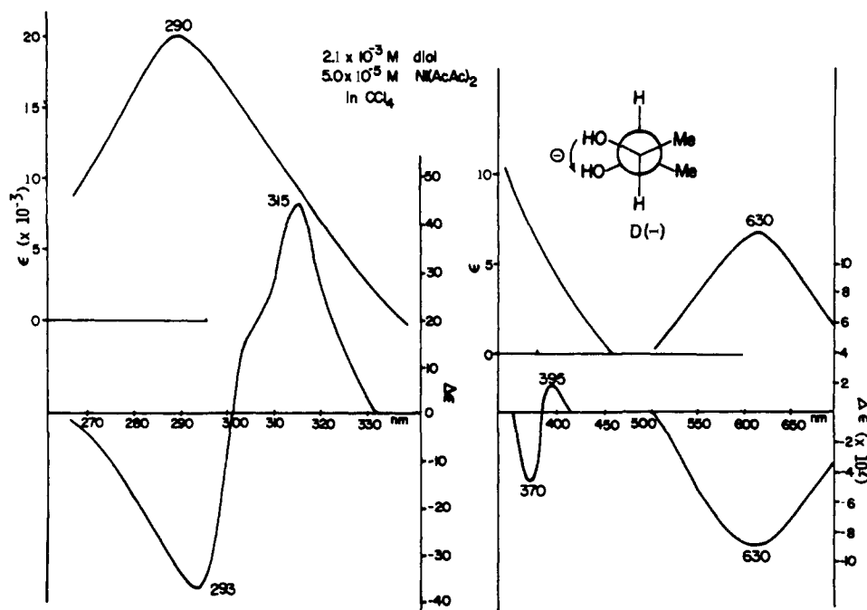
Figure 1. The uv and CD of a mixture of 5.0 \times 10^{-5} M \text{Ni}(\text{acac})_2 and 2.1 \times 10^{-3} M (2R,3R) -butane-2,3-diol in \text{CCl}_4 .
