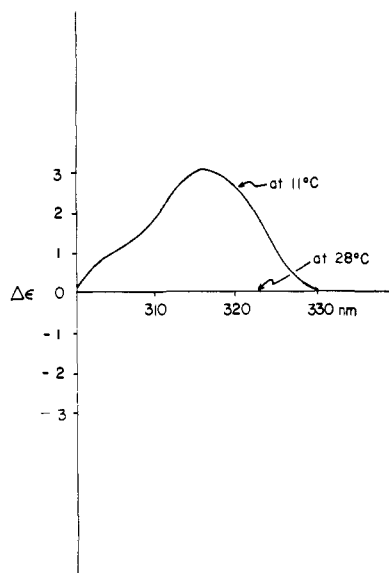
Figure 7. CD of a mixture of \text{Ni}(\text{acac})_2 ( 5.0 \times 10^{-5} M ) and (2R,3R) -butane-2,3-diol ( 3.5 \times 10^{-4} M ) at 28^\circ (baseline) and 11^\circ (curve) in \text{CCl}_4 .
