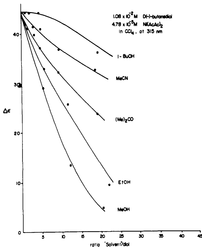
Figure 9. CD observed at 315 nm, when various competing solvents are added to a mixture of 1.08 \times 10^{-2} M (2R,3R) -butane-2,3-diol and 4.78 \times 10^{-5} M \text{Ni}(\text{acac})_2 in \text{CCl}_4 .
